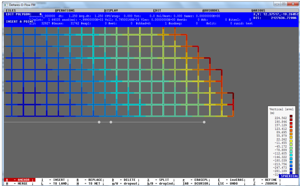
Figure 5: View on the Delft3D grid, visualized in the DFM development environment, as well as a polyline at one of the three boundaries of the example model. The colors visualize the bathymetry.
