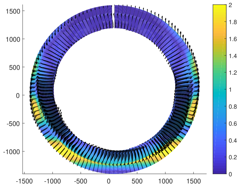
Figure 6.9: Snapshot of the RMS wave height and the flow velocity field in the last time step
