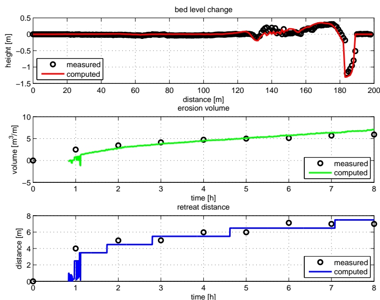
Figure 3.24: Morphodynamics during test 2E
