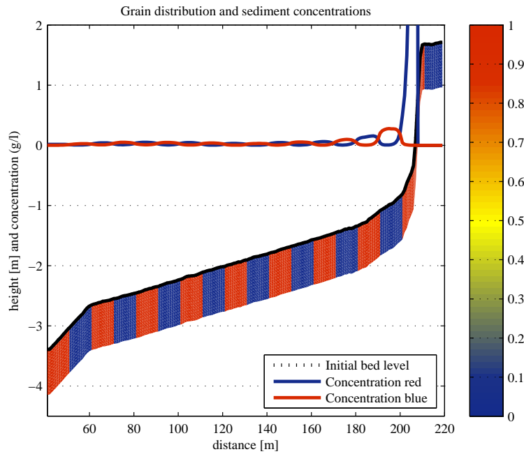
Figure 6.6: Initial bathymetry and sediment distribution
