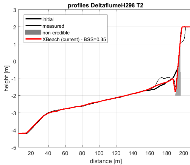
Figure 3.21: Profile development during test T2
