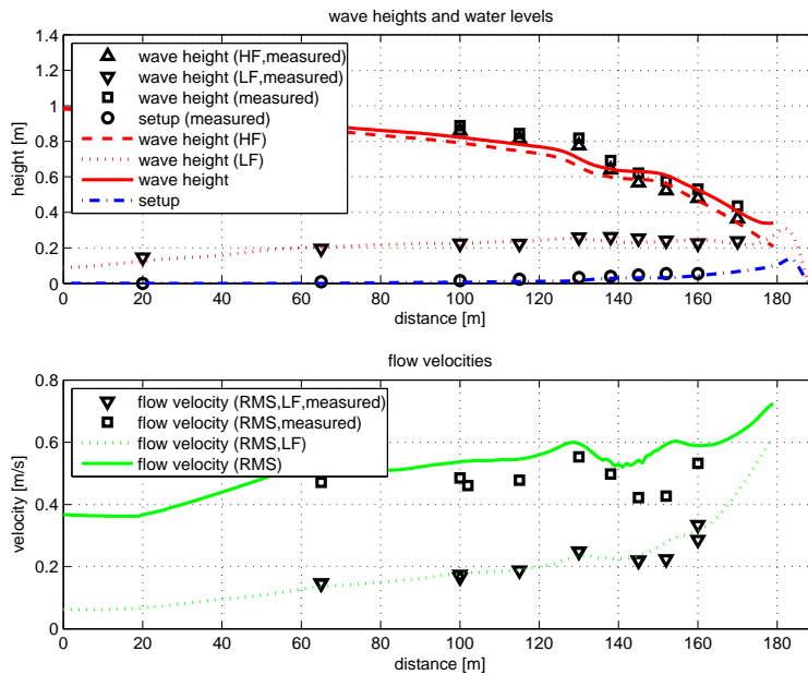
Figure 3.23: Hydrodynamics during test 2E
