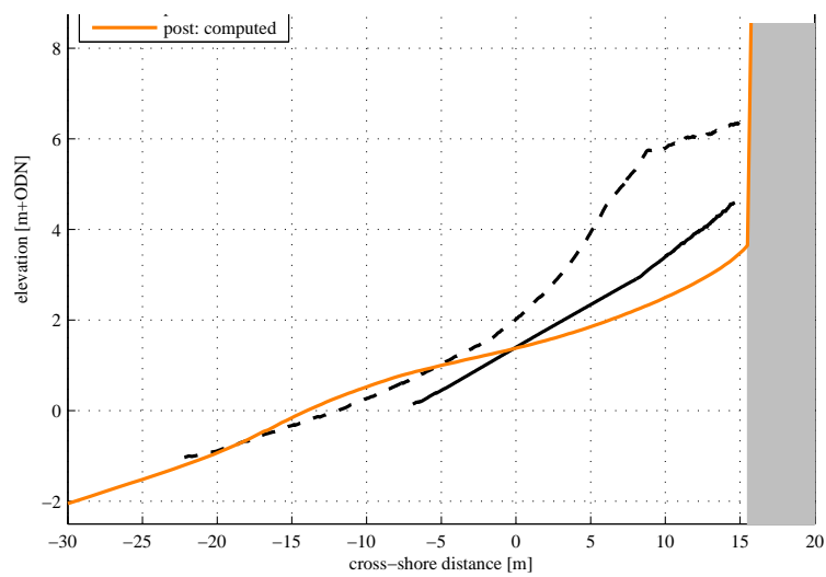
Figure 6.2: Profile development for Chesil Beach
