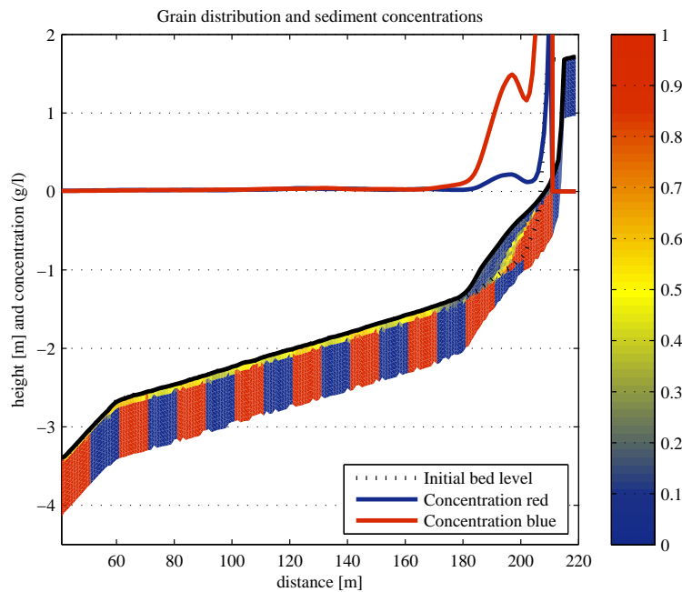
Figure 6.7: Final bathymetry and sediment distribution
