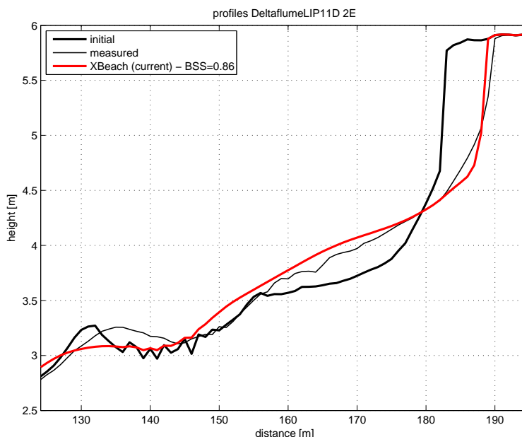
Figure 3.25: Profile development during test 2E
