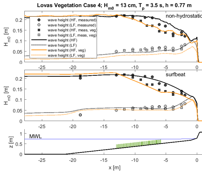
Figure 6.11: Significant high-frequency (sea-swell) and low-frequency (infragravity) wave height computed with XBeach nonhydrostatic (top panel) and surfbeat mode (middle panel) without (black) and with vegetation (orange) for case 4 reported by Lovas (2000). Measurements are indicated with the black and grey symbols (respectively, without and with vegetation)
