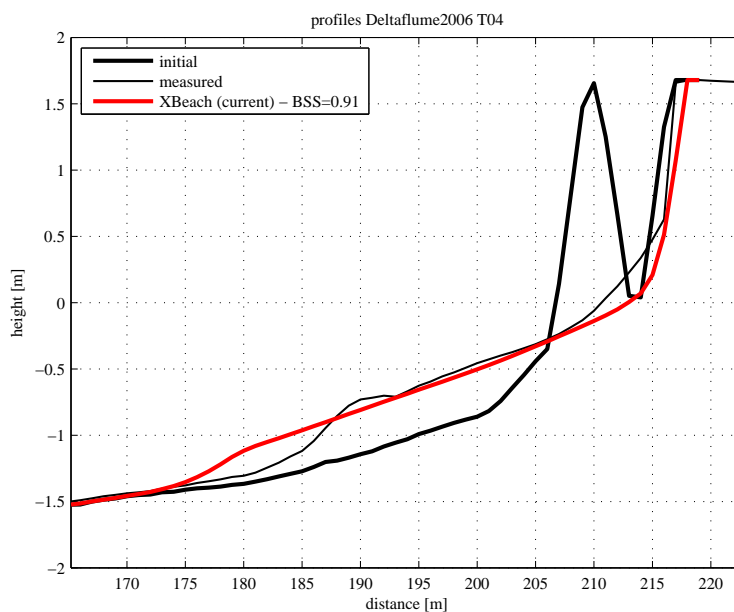
Figure 3.54: Profile development during test T04
