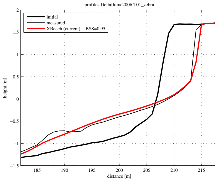
Figure 6.8: Profile development
