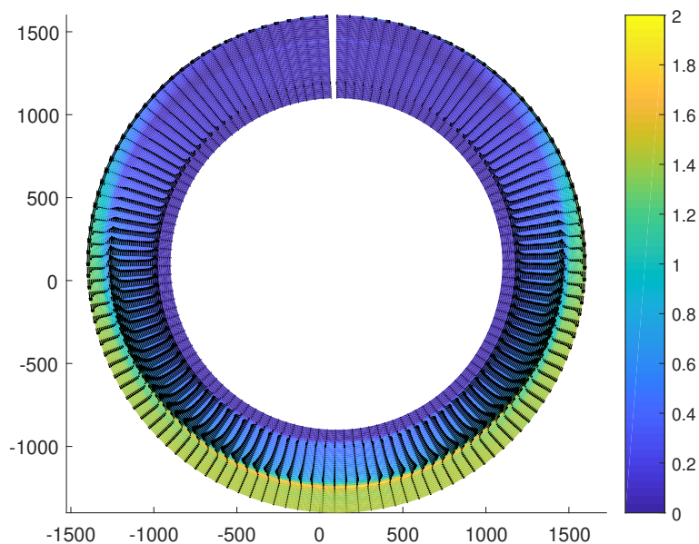
Figure 6.10: Mean values of the RMS wave height and the flow velocity field
