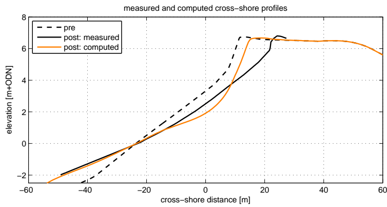
Figure 6.1: Profile development for Slapton Sands
