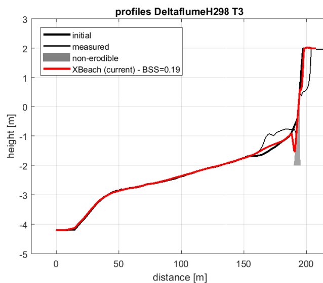
Figure 3.22: Profile development during test T3
