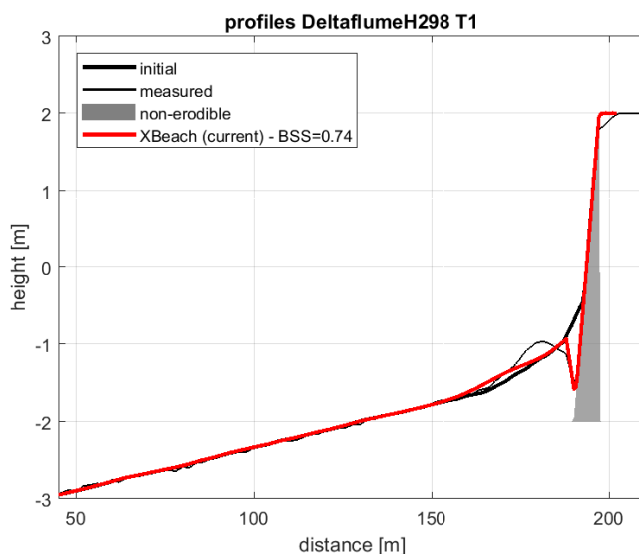
Figure 3.20: Profile development during test T1
