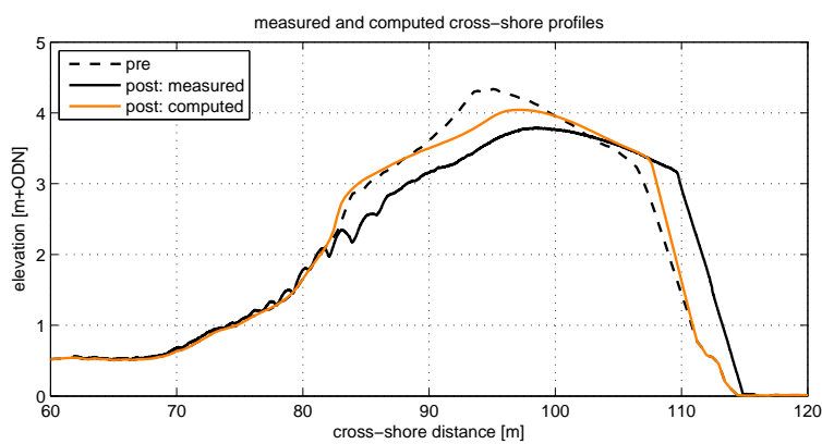
Figure 6.3: Profile development for test E10 of the Bardex experiment
