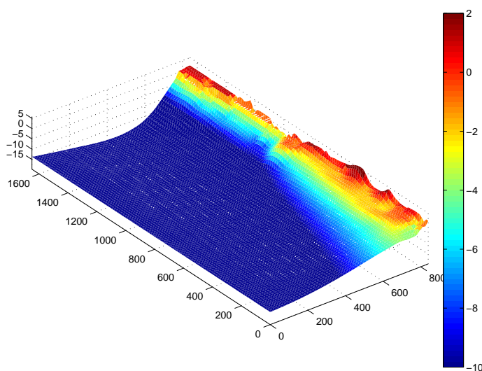
Figure 6.4: Final bathymetry
