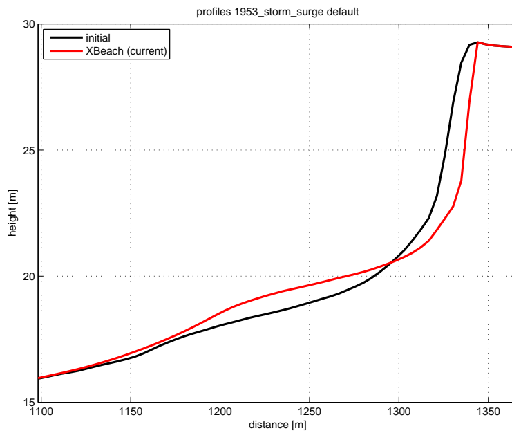
Figure 4.2: Profile development
