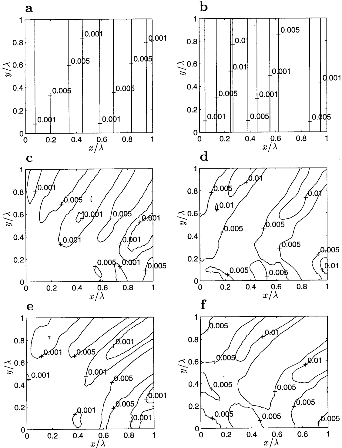
Figure 5: Reflection errors vs (x/\lambda, y/\lambda) for wave amplitude A/h_0 = 0.01 using (16) (a) linear scheme, \theta_i = 0 , at t^n = T ; (b) nonlinear scheme, \theta_i = 0 , at t^n = T ; (c) linear scheme, \theta_i = \frac{\pi}{6} , at t^n = T/\cos \frac{\pi}{6} ; (d) nonlinear scheme, \theta_i = \frac{\pi}{6} , at t^n = T/\cos \frac{\pi}{6} ; (e) linear scheme, \theta_i = \frac{\pi}{4} , at t^n = T/\cos \frac{\pi}{4} ; (f) nonlinear scheme, \theta_i = \frac{\pi}{4} , at t^n = T/\cos \frac{\pi}{4} .
