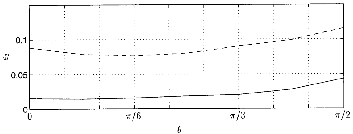
Figure 8: Reflection error vs. angle of incidence \theta_i for A/h_o = 0.1 . First order BC (dashed line), second order BC (solid line).
