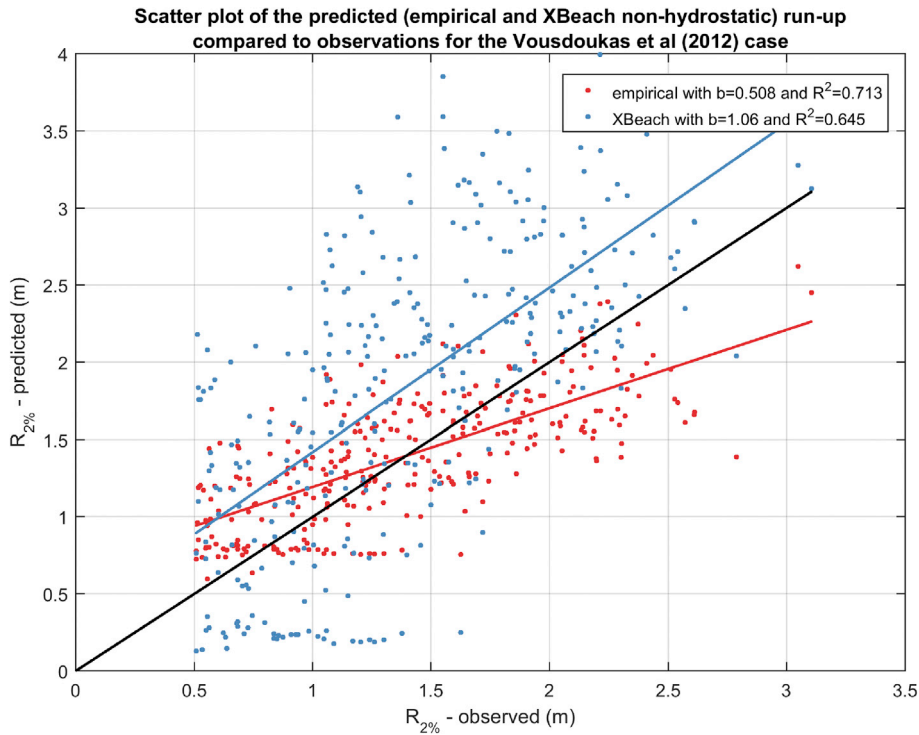
Fig. 15. Predicted vs. observed R_{2\%} run-up height and regression curves; 1D non-hydrostatic.
