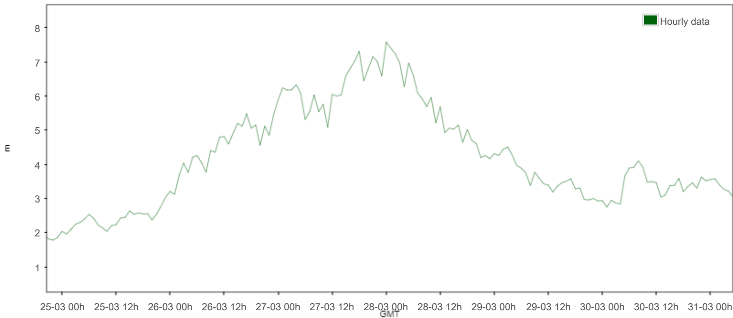
i Villano-Sisargas Buoy, Significant Wave Height.
