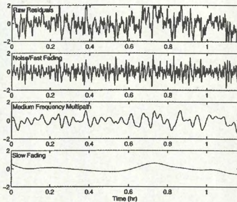
Figuur 9 Multipad frequenties ( <1m , 1<t<8m , <8m )
