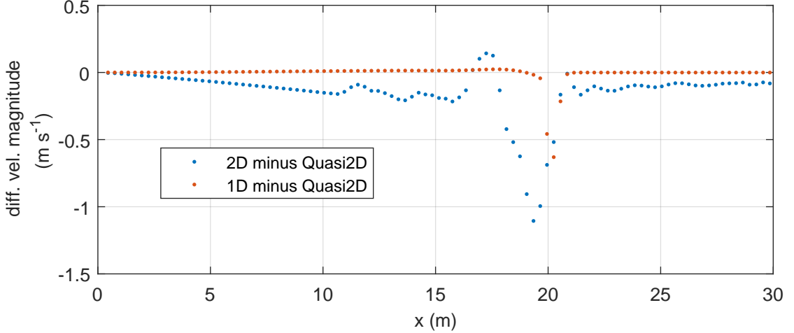
Engelund-Hansen: vel. magnitude differences
