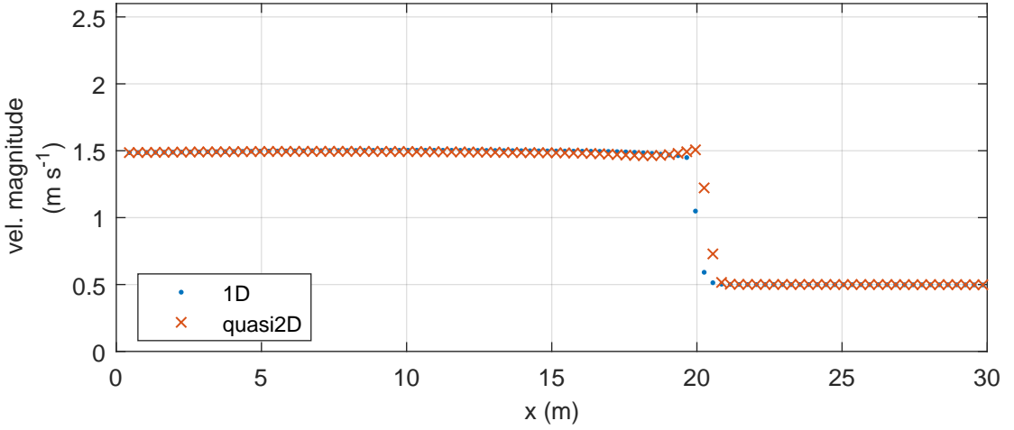
Engelund-Hansen: vel. magnitude 2D comparison
