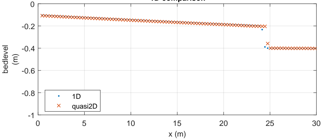
Engelund-Hansen: bedlevel 2D comparison
