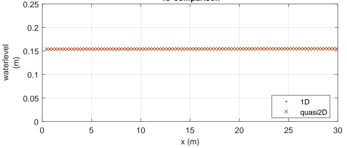
Engelund-Hansen: waterlevel 2D comparison
