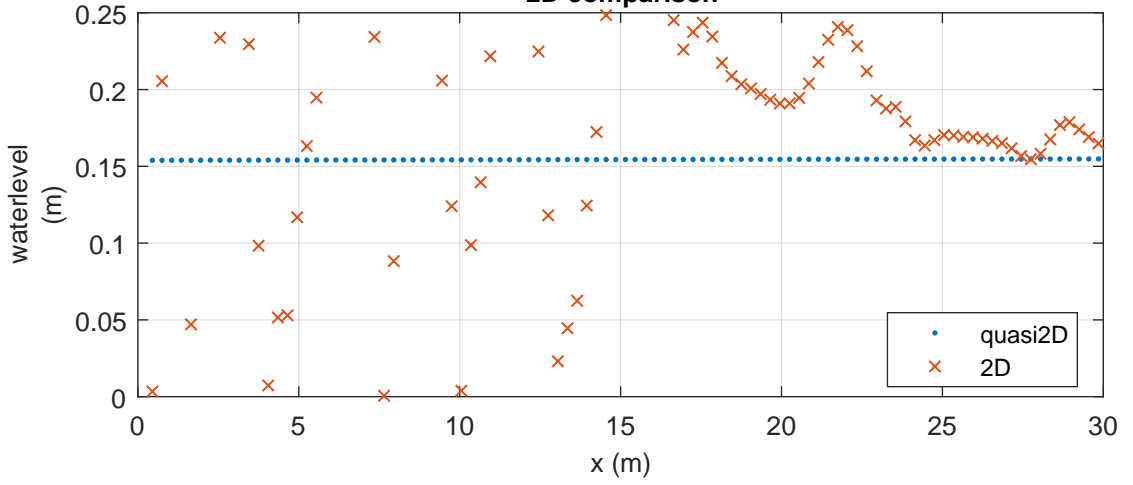
Engelund-Hansen: waterlevel differences
