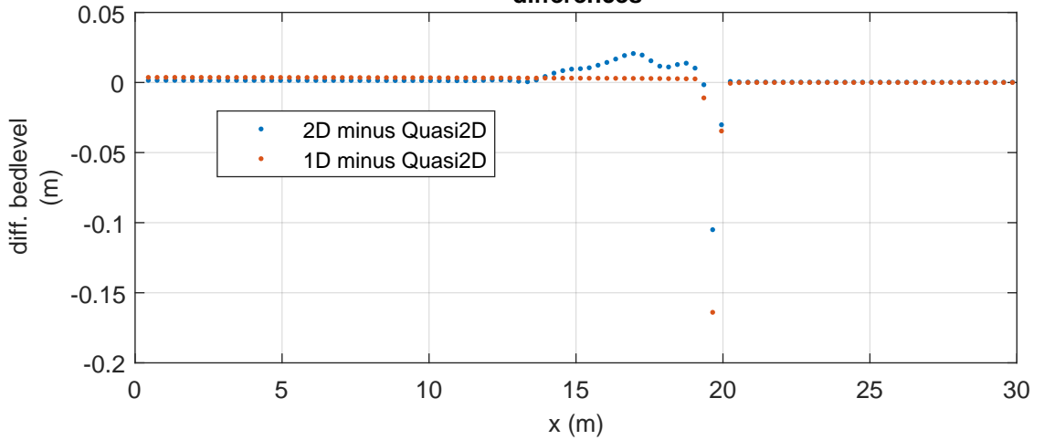
Engelund-Hansen: bedlevel differences
