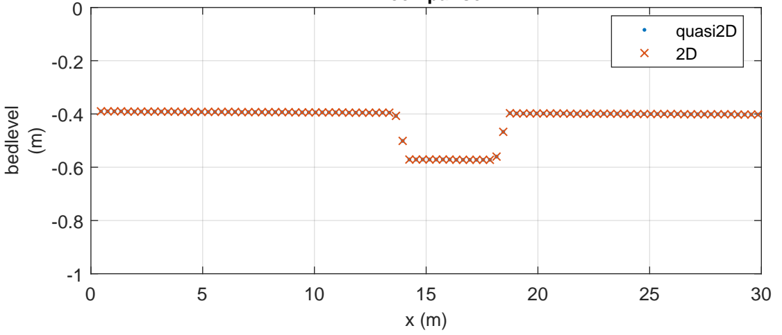
Engelund-Hansen: bedlevel differences
