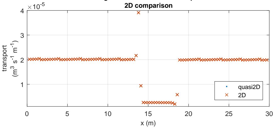
Engelund-Hansen: Total transport differences
