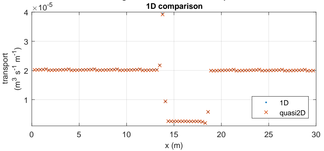
Engelund-Hansen: Total transport 2D comparison
