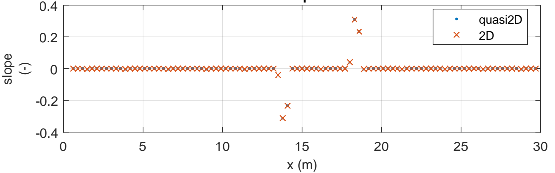
Engelund-Hansen: slope differences
