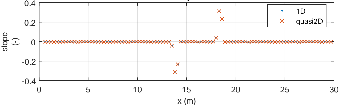
Engelund-Hansen: slope 2D comparison
