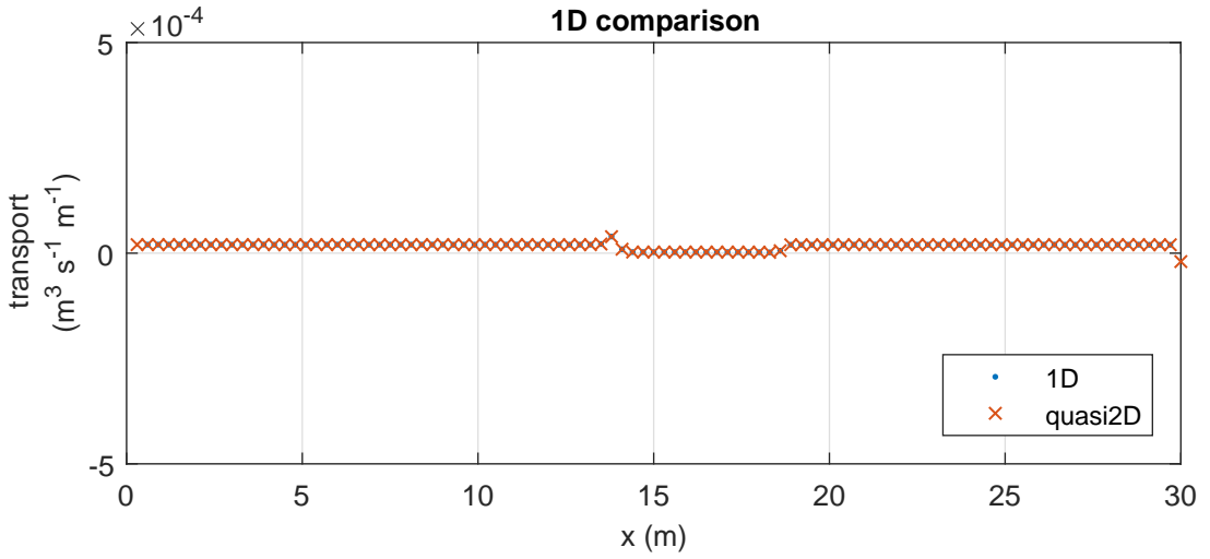
Engelund-Hansen: bedload 2D comparison
