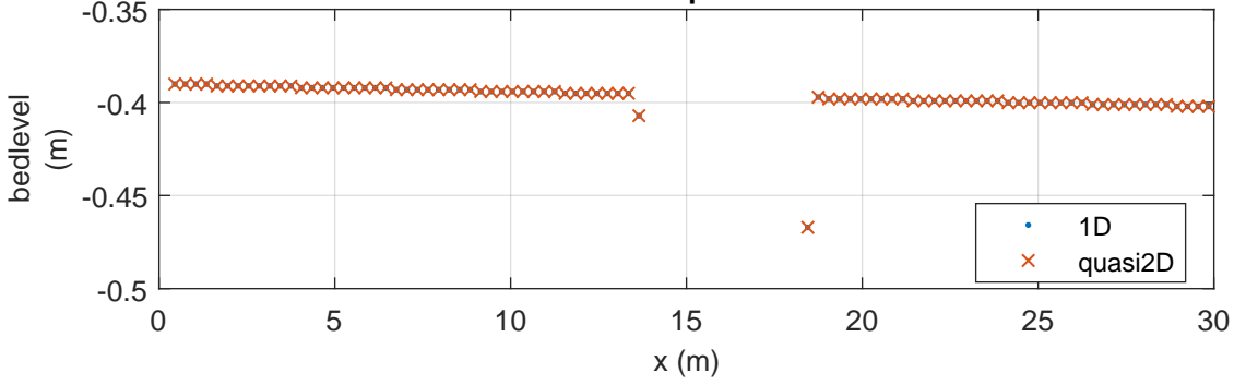
Engelund-Hansen: bedlevel 2D comparison
