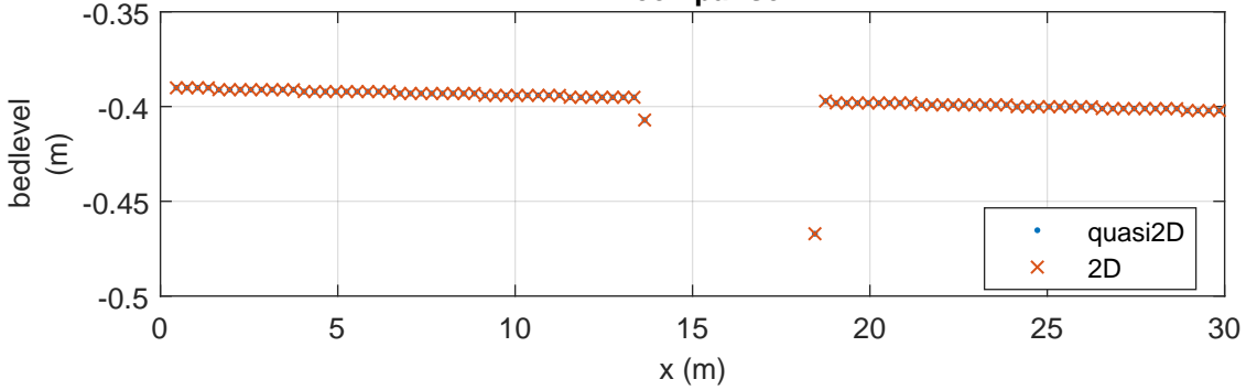
Engelund-Hansen: bedlevel differences
