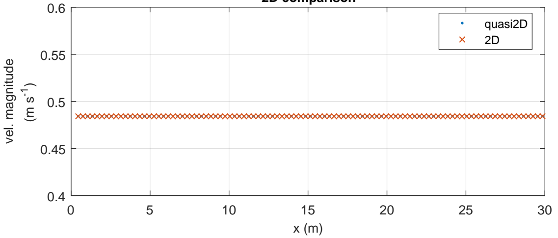
Engelund-Hansen: vel. magnitude differences
