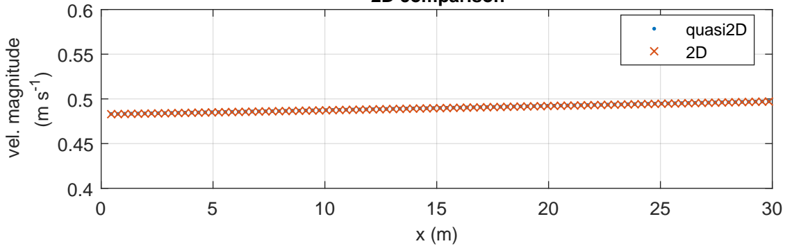
Engelund-Hansen: vel. magnitude differences
