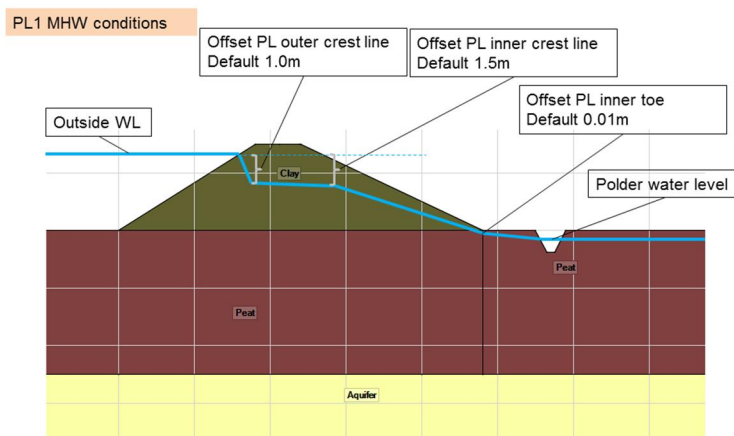
Figure 2.5 Phreatic line during extreme (MHW) conditions
