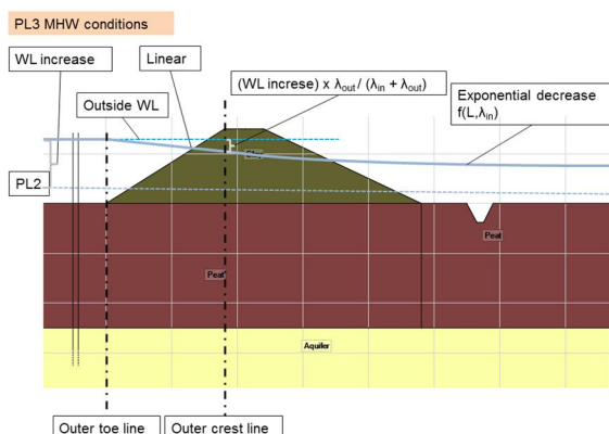
Figure 2.7 Pore pressure aquifer during extreme conditions
