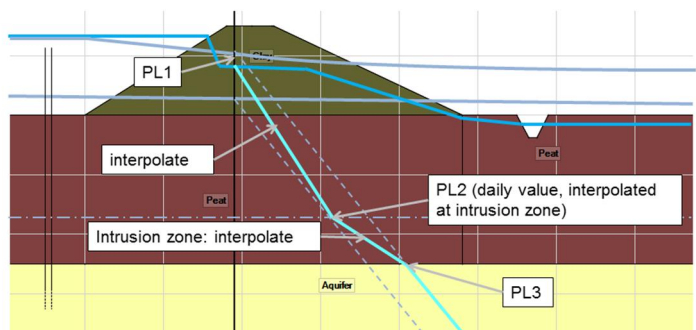
Figure 2.9 Pore water pressure during extreme conditions
