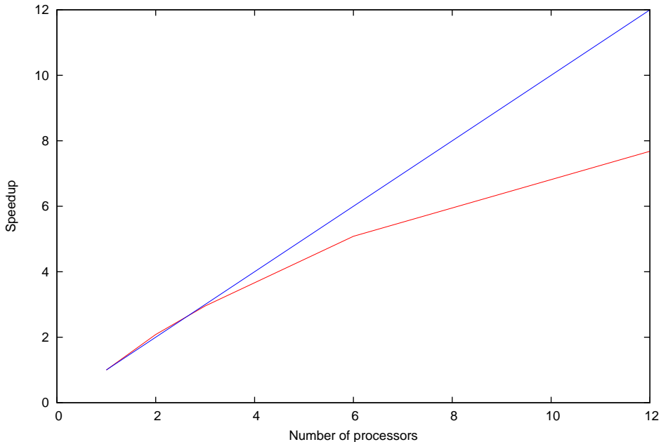
Lotos-Euros; Ensemble of 24 model on ASTER 30x30x4 mesh 24 hour simulation
