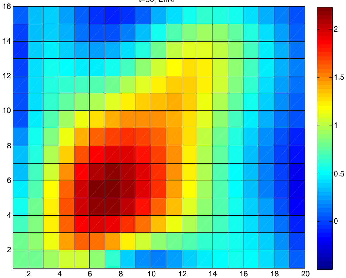
t=50, EnKF
