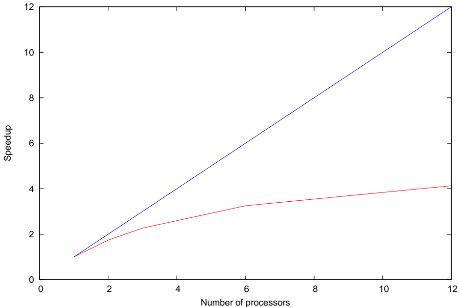
Lotos-Euros; Ensemble of 24 model on ASTER 60x60x4 mesh 24 hour simulation
